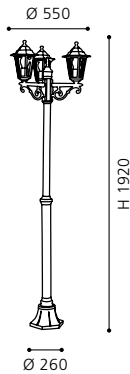
floor luminaire; cast aluminium, white / glass, clear Stehleuchte; Aluguss, weiss / Glas, klar lampadaire; aluminium moulé, blanc / verre, clair
